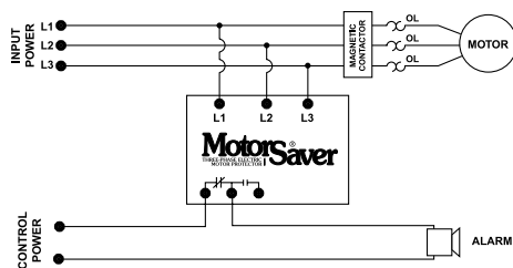
Figure No. 1: Typical Wiring Diagram
