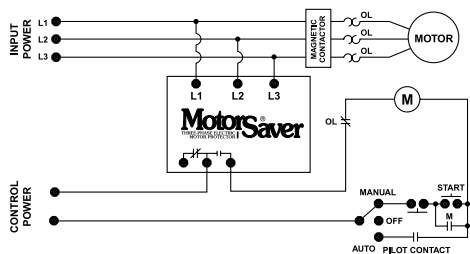
Figure No. 1: Typical Wiring Diagram
